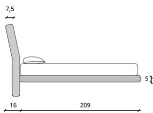
bed with curved headboard dimensions do not take into account feet
