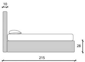
dimensions do not take into account feet you can choose one or both paneling (right or left) including storage box
